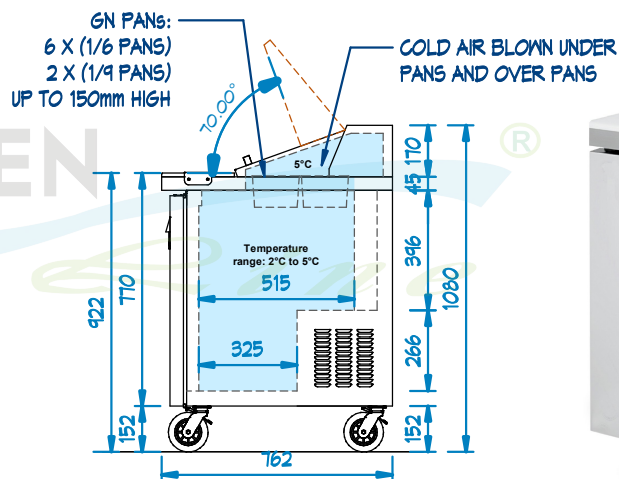
SIDE VIEW scale 1:25 m
