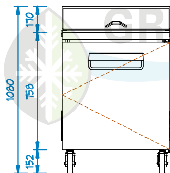
FRONT VIEW scale 1:25 m
