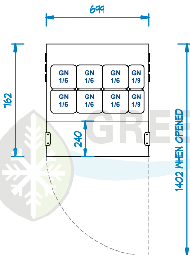
TOP VIEW scale 1:25 m
