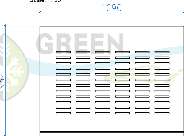
2 FRONT VIEW
